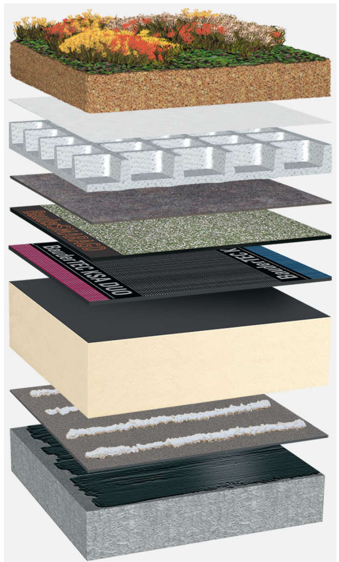
Systemaufbau: BG_PIR-FA_S_01_G75
