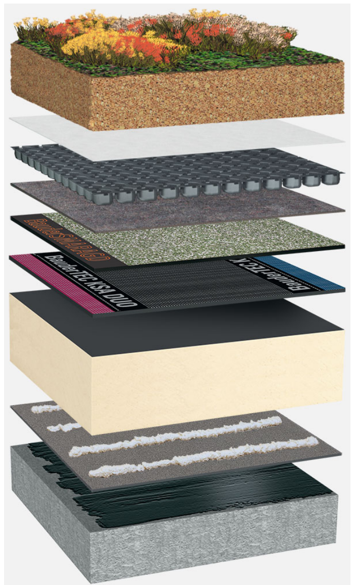
Systemaufbau: BG_PIR-FA_S_01_G125
