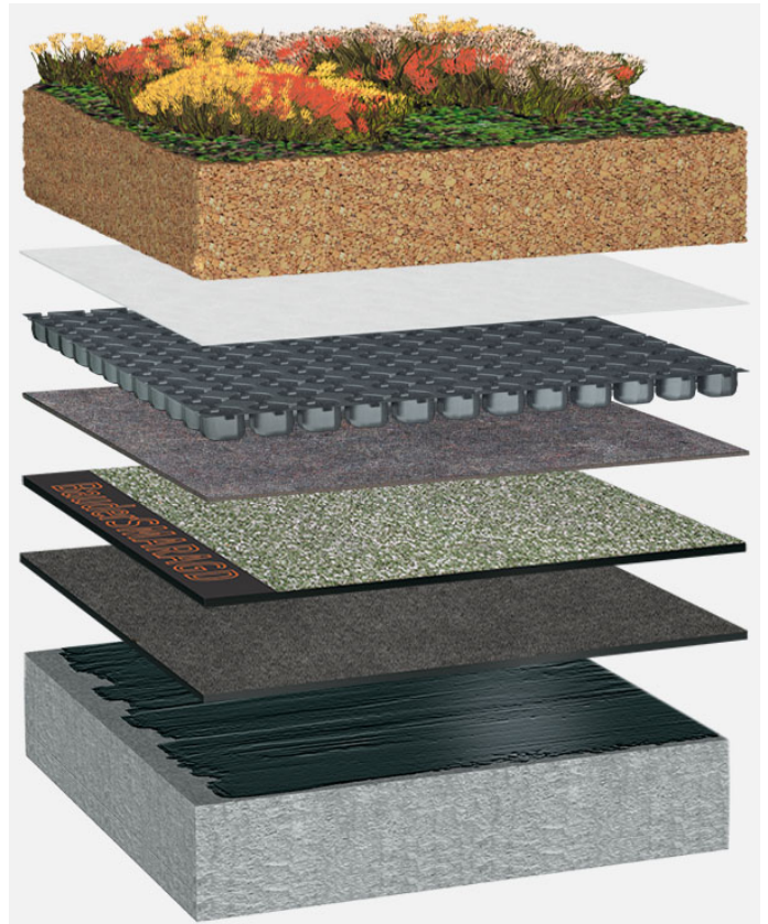
Systemaufbau: BG_S_01_G125
